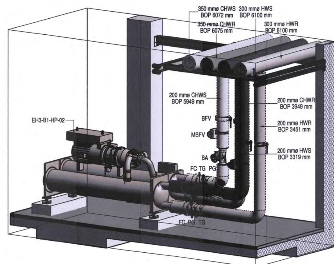
D HEAT PUMP DETAILS 0007
