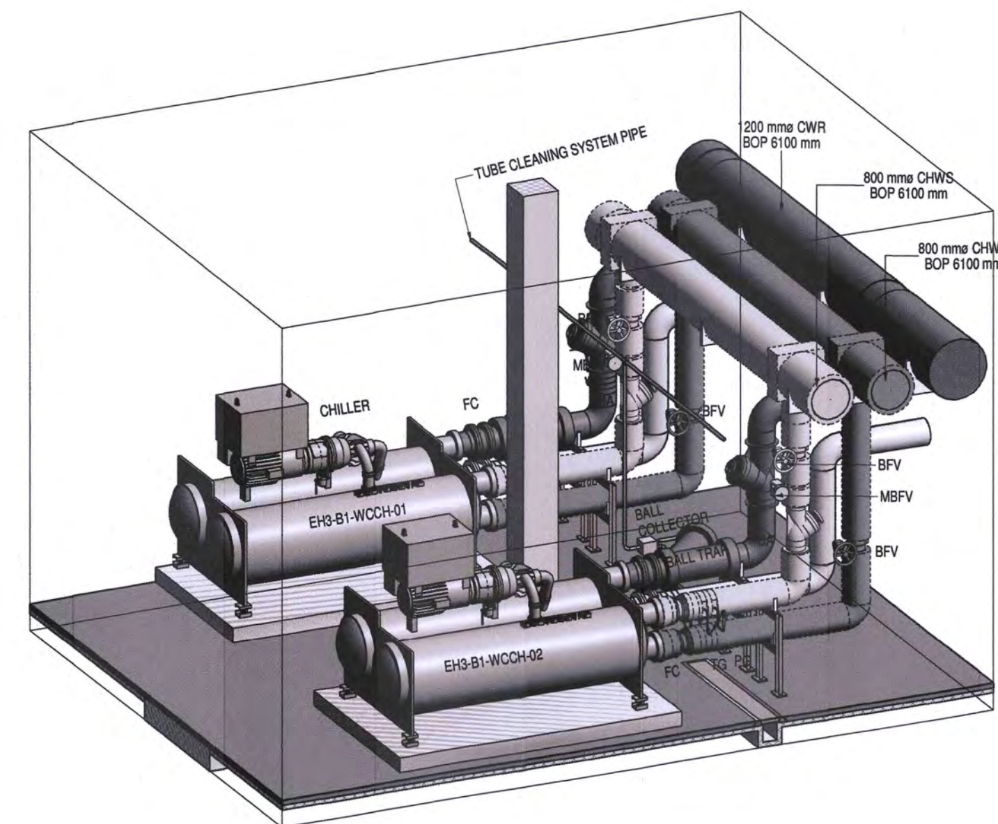
C 3D VIEW OF CHILLER CONNECTION DETAILS 0007
