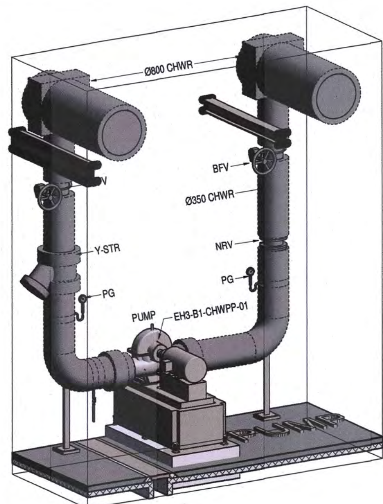
B PUMP CONNECTION DETAILS 0007
