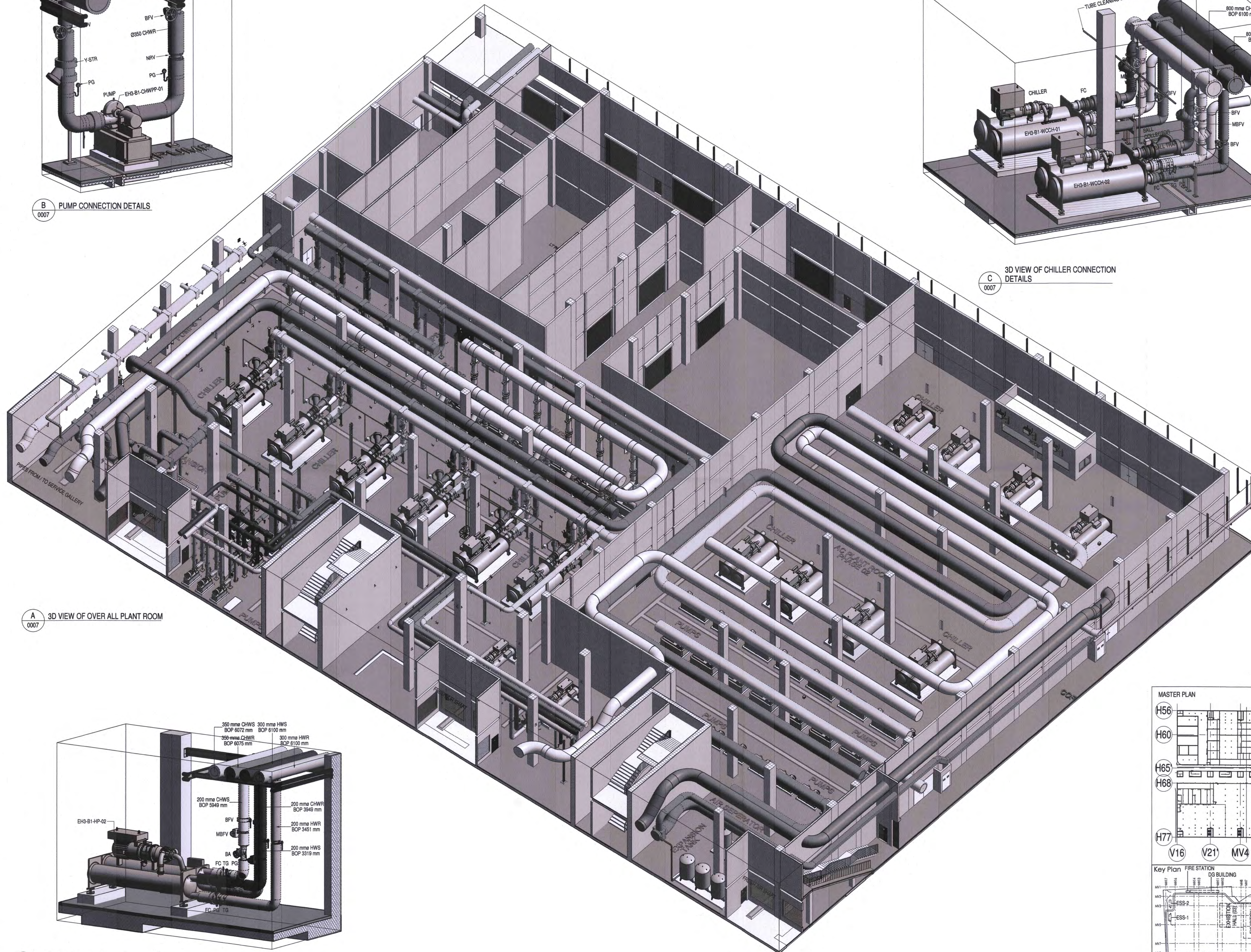
D HEAT PUMP DETAILS 0007
