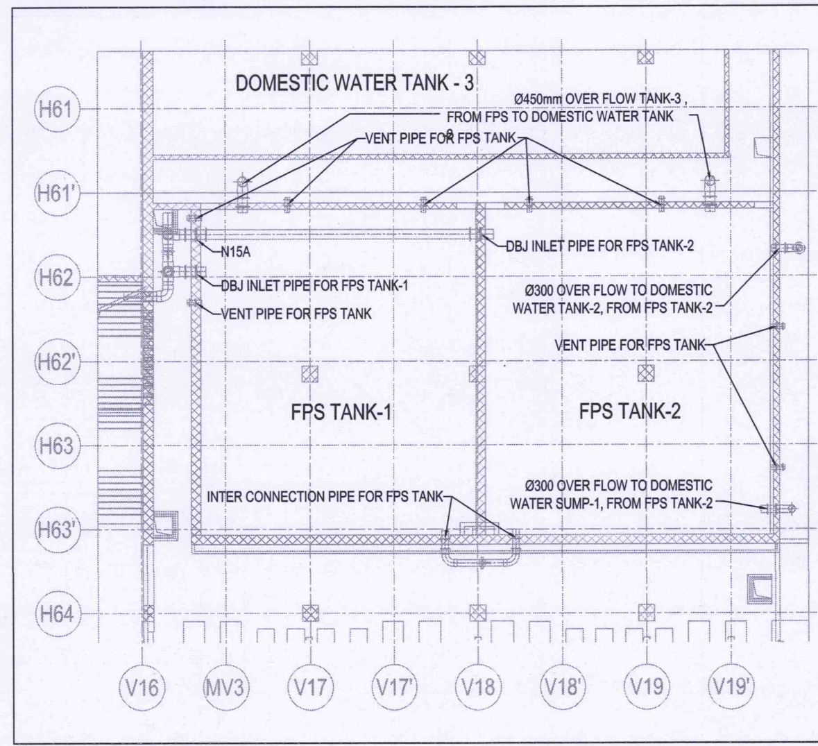
FIRE WATER TANK OVER FLOW DETAILS
